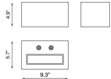
Fixture Dimensions
