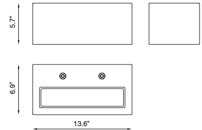
Fixture Dimensions
