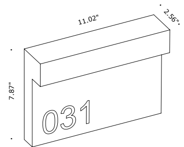
Fixture Dimensions
