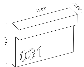
Fixture Dimensions
