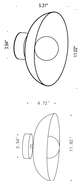
Fixture Dimensions
