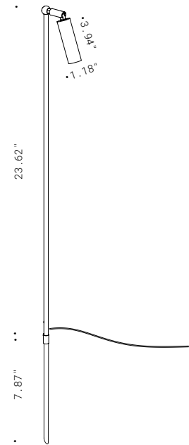
Fixture Dimensions
