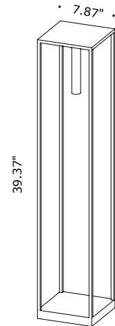
Fixture Dimensions
