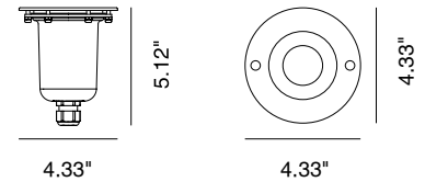
Fixture Dimensions
