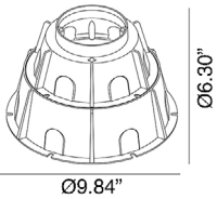
PT52122 Draining Casing for ground recessing
