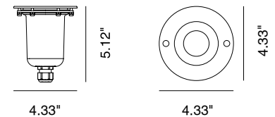
Fixture Dimensions
