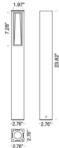
Fixture Dimensions
