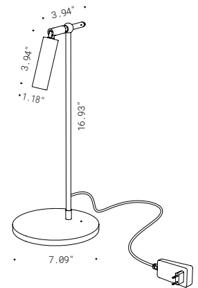
Fixture Dimensions
