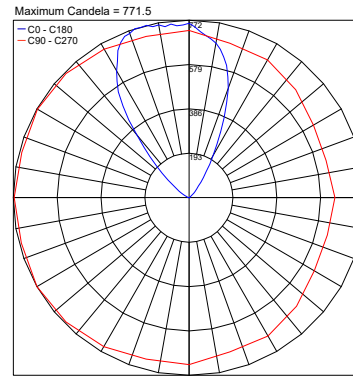
PHOTOMETRIC FILENAME : BASE V02 30K 65° BLACK - PT1022036B.IES
