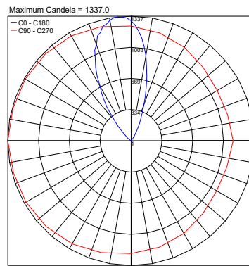
PHOTOMETRIC FILENAME : BASE H02 30K 45° BLACK - PT1024034B.IES
