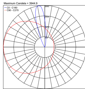
PHOTOMETRIC FILENAME : BASE H02 30K 21° BLACK - PT1024032B.IES
