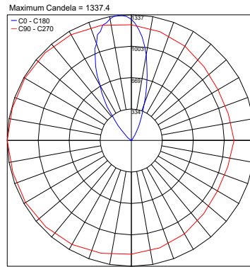
PHOTOMETRIC FILENAME : BASE V02 30K 45° BLACK - PT1022034B.IES
