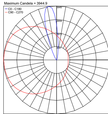
PHOTOMETRIC FILENAME : BASE V02 30K 21° BLACK - PT1022032B.IES
