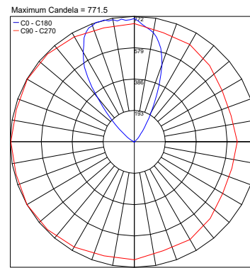
PHOTOMETRIC FILENAME : BASE H02 30K 65° BLACK - PT1024036B.IES
