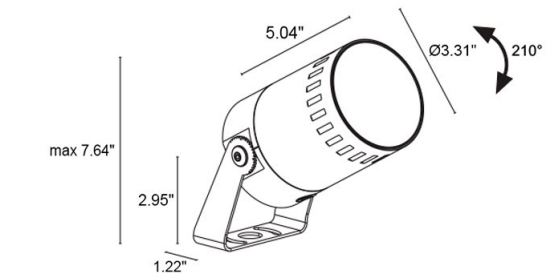
Fixture Dimensions
