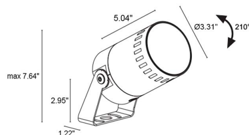
Fixture Dimensions
