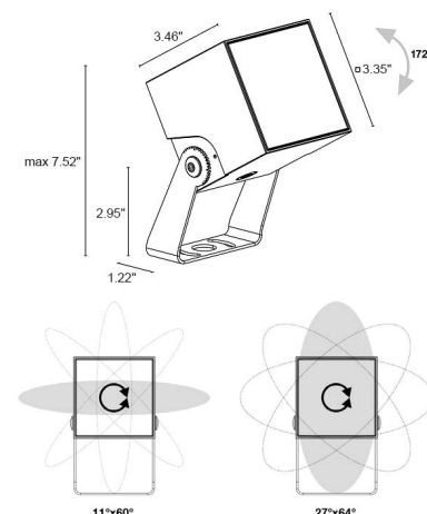
Fixture Dimensions
