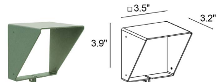
WBA13__ Asymmetric Snoot For Snoots include one of the below finishes: E - White F - Gray H - Anthracite T - Cor-ten 5 - Jasper Green C - Custom RAL
