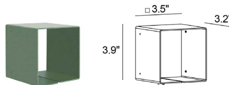
WBA12__ Standard Snoot For Snoots include one of the below finishes: E - White F - Gray H - Anthracite T - Cor-ten 5 - Jasper Green C - Custom RAL
