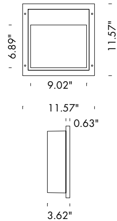
Fixture Dimensions
