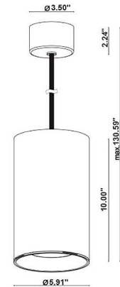
Fixture Dimensions
