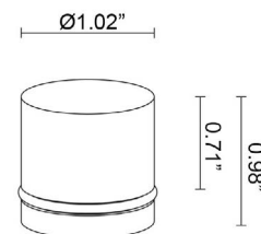
Fixture Dimensions
