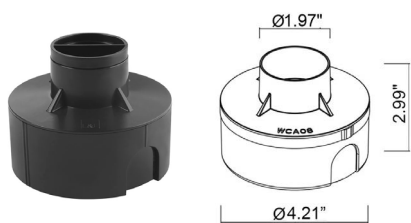
WCA08 Outer Casing For in-grade use
