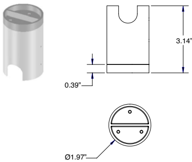
AH-00016 Core Drilled Application Sleeve
