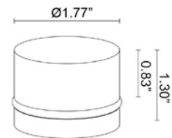
Fixture Dimensions
