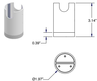
WCA08 Outer Casing For in-grade use
