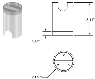
WCA08 Outer Casing For in-grade use
