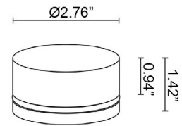
Fixture Dimensions
