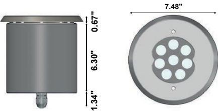
Fixture Dimensions
