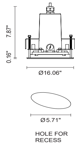
Fixture Dimensions
