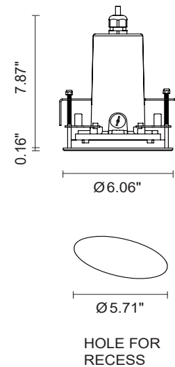
Fixture Dimensions
