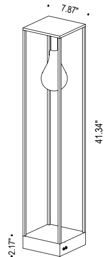
Fixture Dimensions
