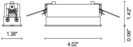
Fixture Dimensions
