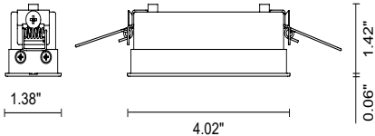
Fixture Dimensions
