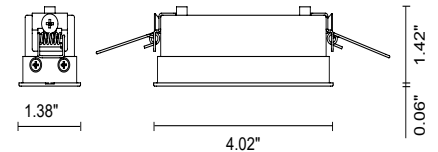
Fixture Dimensions
