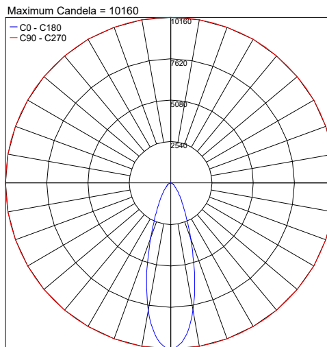
PHOTOMETRIC FILENAME : NAIL 3000K-30°-36W-TRANSPARENT-GLASS.JIES
