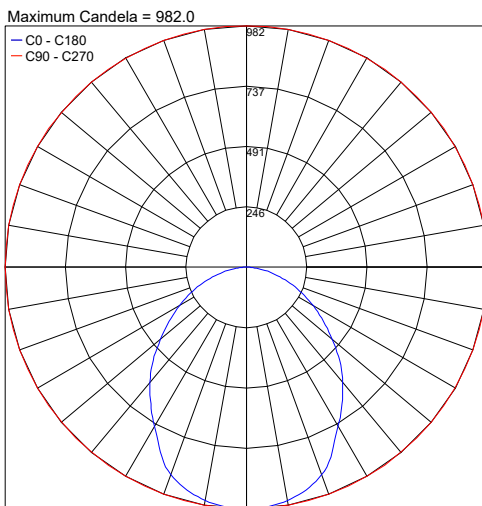
PHOTOMETRIC FILENAME : NAIL 3000K-DIFFUSED-22W-SAND-BLASTED.JIES
