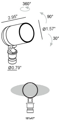
Fixture Dimensions
