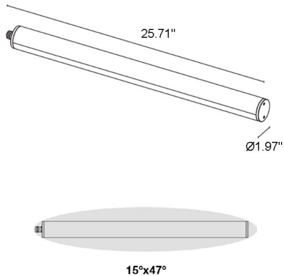
Fixture Dimensions
