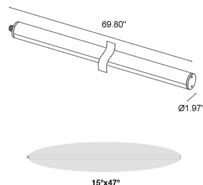
Fixture Dimensions
