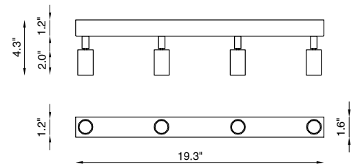
Fixture Dimensions
