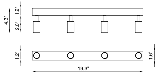
Fixture Dimensions
