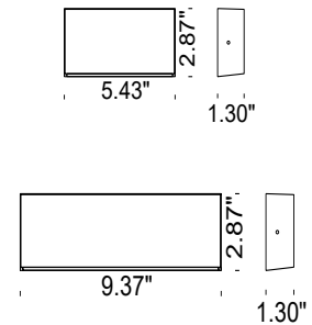
Fixture Dimensions
