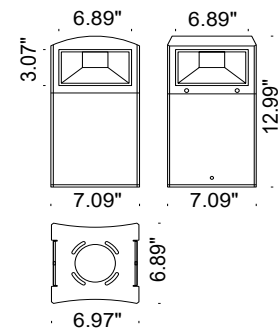
Fixture Dimensions
