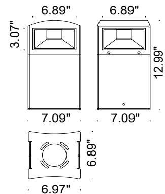
Fixture Dimensions
