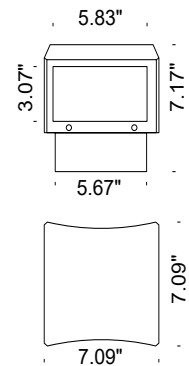
Fixture Dimensions
