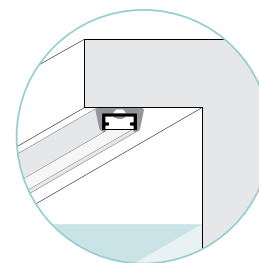
OUT-S-9.5x6.5.F/W Flexible Silicone Outercase L=16.4"
