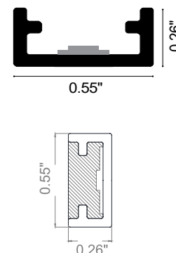
Fixture Dimensions
