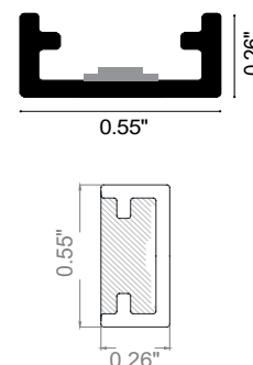
Fixture Dimensions
