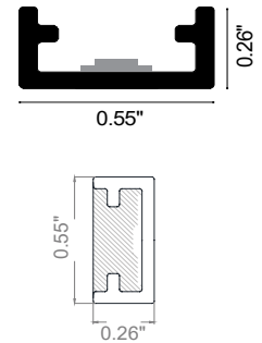
Fixture Dimensions
