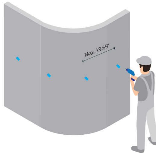
02. By placing the clip on the installation plane, fasten it to the same with the countersunk screw.
