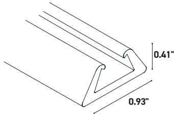
Silicone outercase to press-in the LED strip
