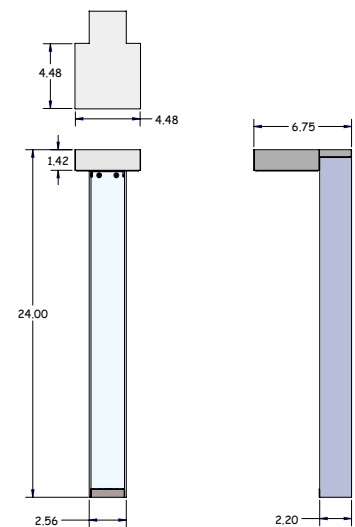
Fixture Dimensions
