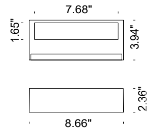
Fixture Dimensions
