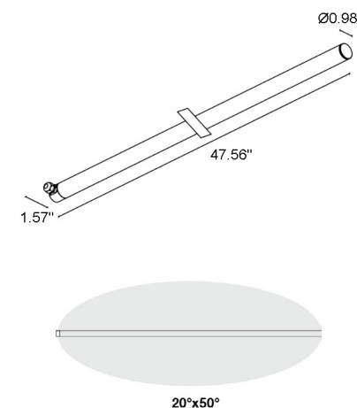
Fixture Dimensions
