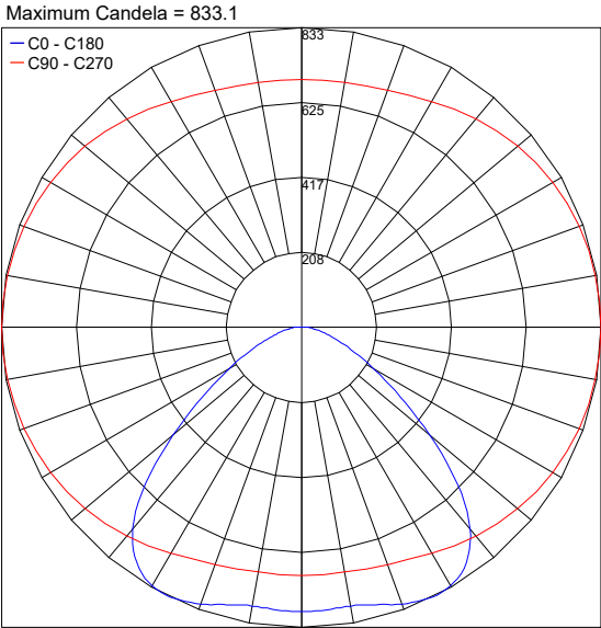
PHOTOMETRIC FILENAME : TREVI_2.0_D_3000K_21W_24VDC.IES
